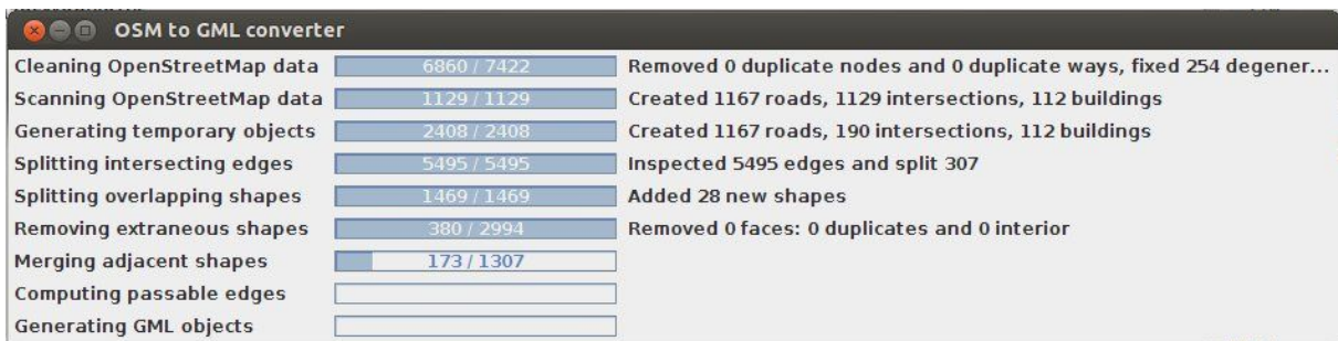
Figure 12. Converter osm2gml Running
